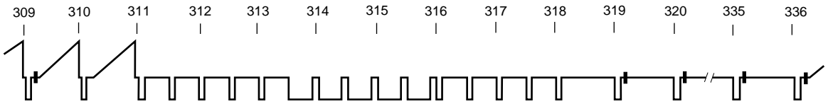
(b) 4th field CVBS output signal
