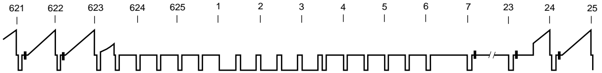
(a) 3rd field CVBS output signal
